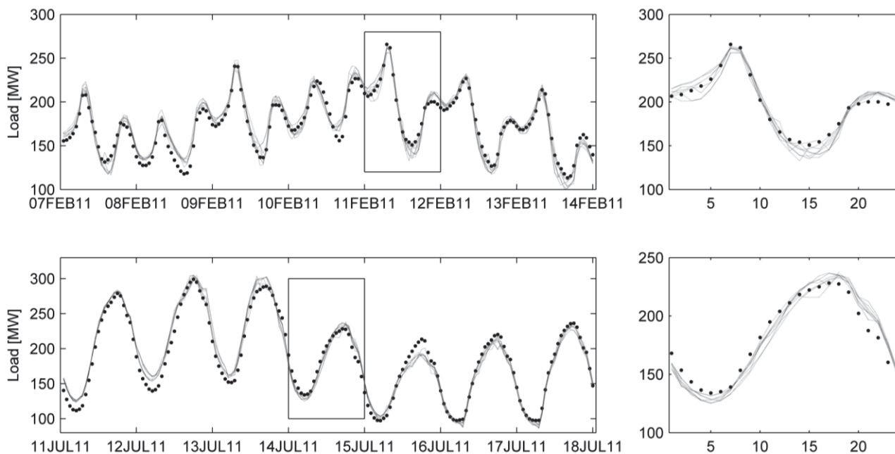
Fig. 2. Actual load (black dots) and 8 sister forecasts (gray lines) in a winter week (upper left) and a summer week (bottom left). The right panels zoom in on two days, which are indicated by rectangles in the left panels. Since the sister forecasts are similar by nature, the differences between them are hardly visible.
