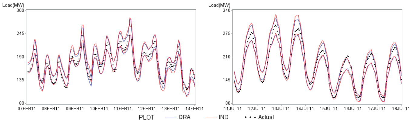
Fig. 3. Actual load (black dots) and two sets of 90% PIs (blue – QRA, red – IND) in the same winter week (left) and the same summer week (right) as in Fig. 2. While both PIs are able to cover most of actual values, the PIs of QRA are narrower than those of the individual model.
