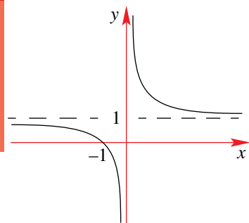
Asymptotes: vertical, x = 0 horizontal, y = 1
