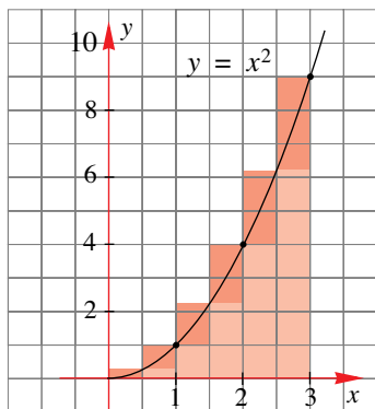
5 lower & 6 upper rectangles
